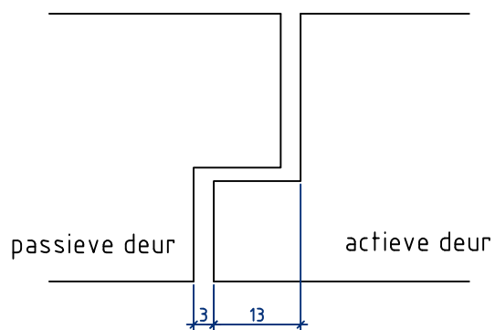
Detail 3: sponning-contrasponning
