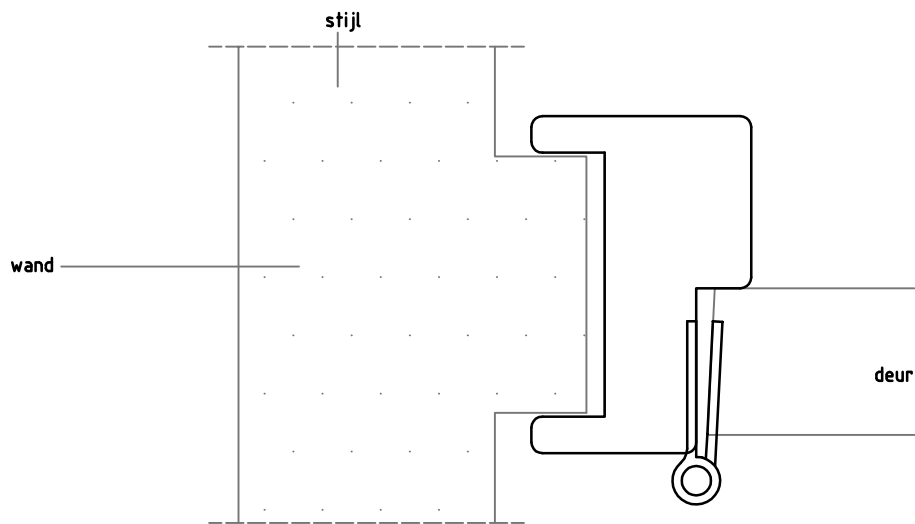
Detail 1: stijl
