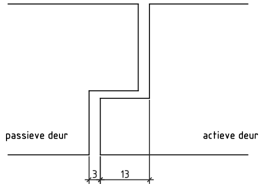
Detail 3: sponning-contrasponning
