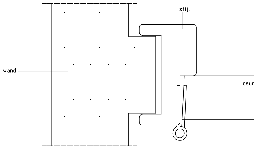
Detail 1: stijl
