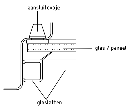
Detail 6: glaslat
