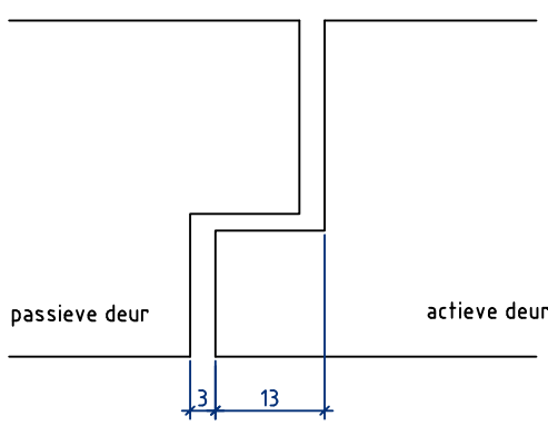
Detail 5: sponning-contrasponning
