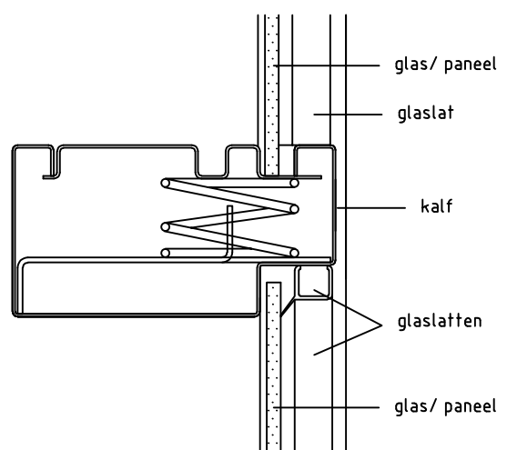
Detail 7: kalf
