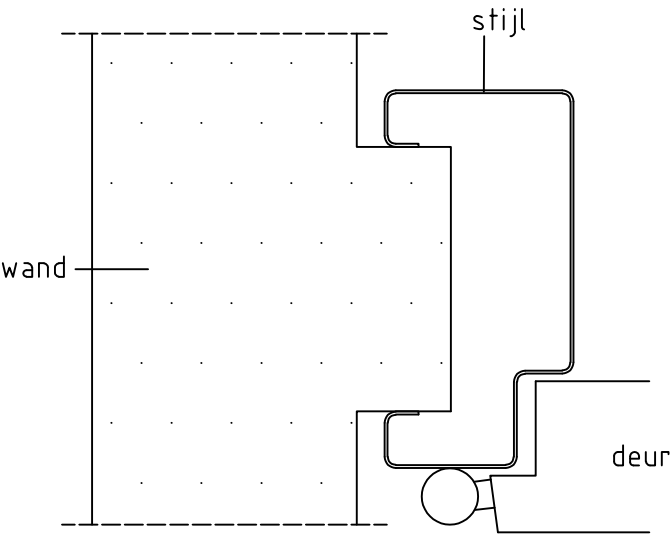
Detail 1: stijl
