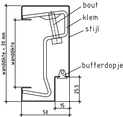
Detail 2: klem
