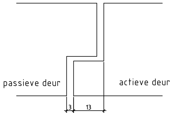
Detail 5: sponning-contrasponning
