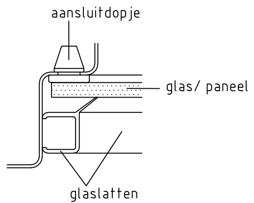
Detail 6: glaslat
