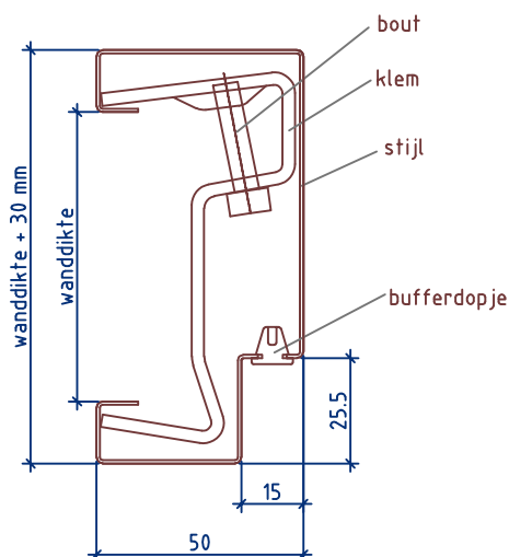
Detail 2: klem
