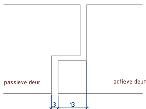
Detail 5: sponning-contrasponning
