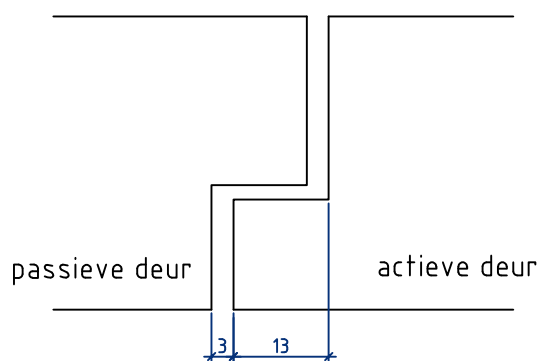
Detail 3: sponning-contrasponning
