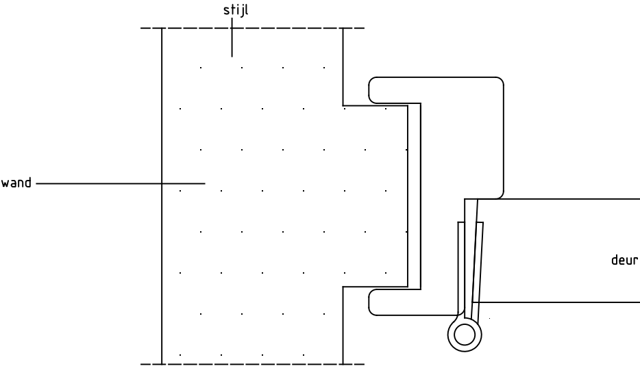
Detail 1: stijl
