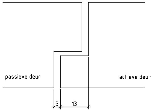
Detail 3: sponning-contrasponning
