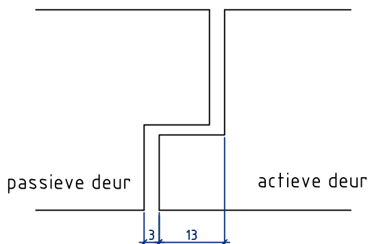
Detail 3: sponning-contrasponning
