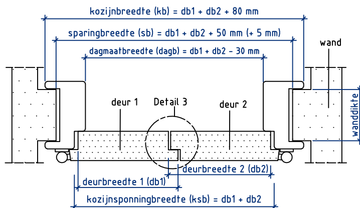
Doorsnede AA spoonning/contrasponning
