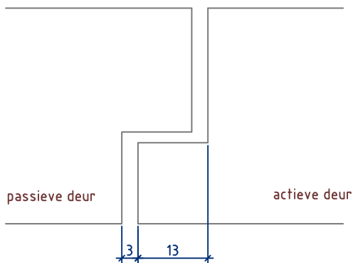
Detail 5: sponning-contrasponning
