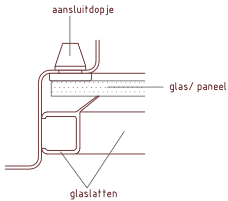
Detail 7: glaslat
