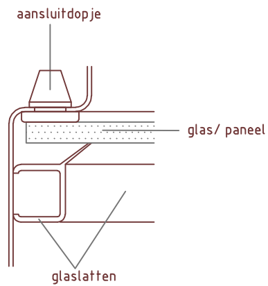
Detail 6: glaslat
