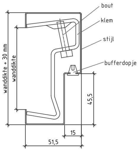
Detail 2: klem
