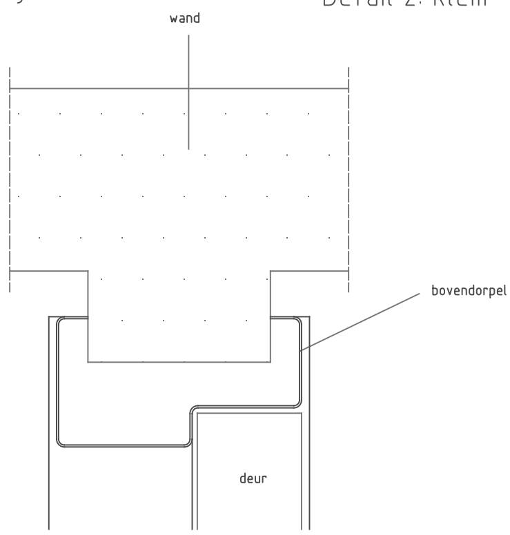
Detail 2: klem
