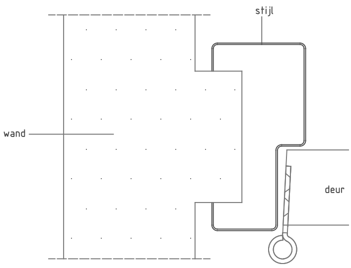
Detail 1: stijl
