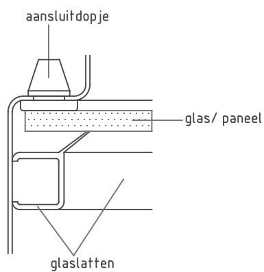
Detail 4: sponning-contrasponning
