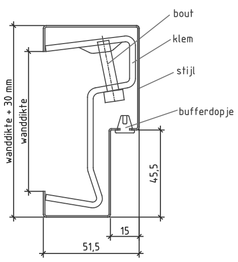
Detail 2: klem
