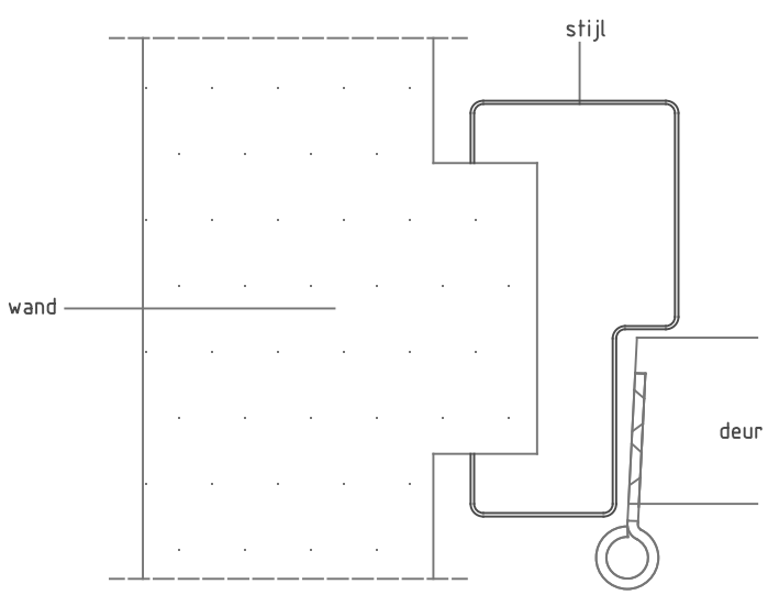
Detail 1: stijl
