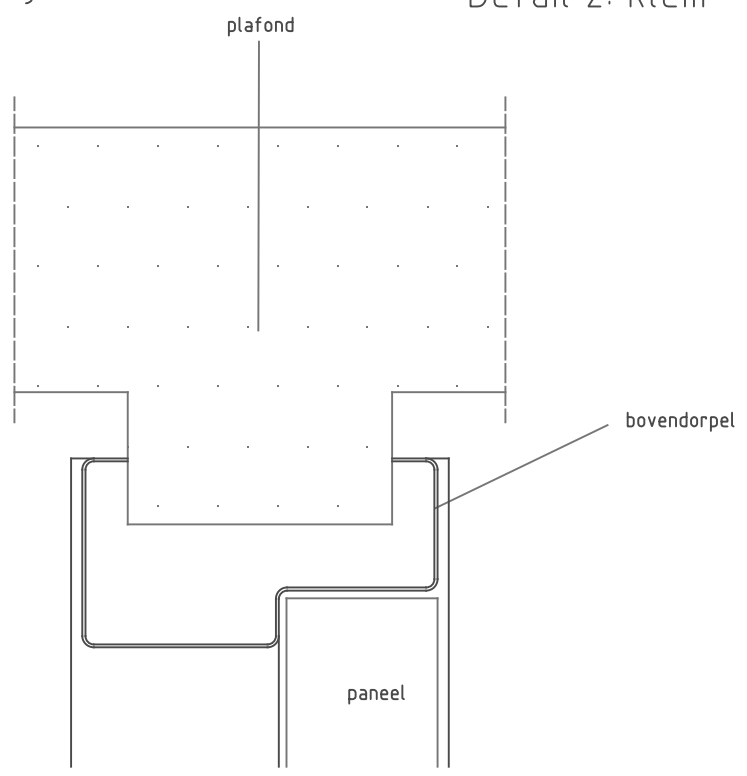
Detail 2: klem
