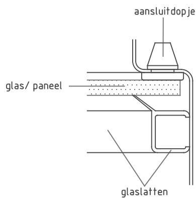
Detail 5: glaslat
