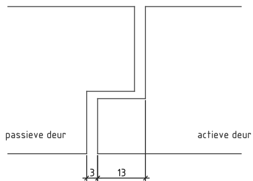
Detail 4: sponning-contrasponning
