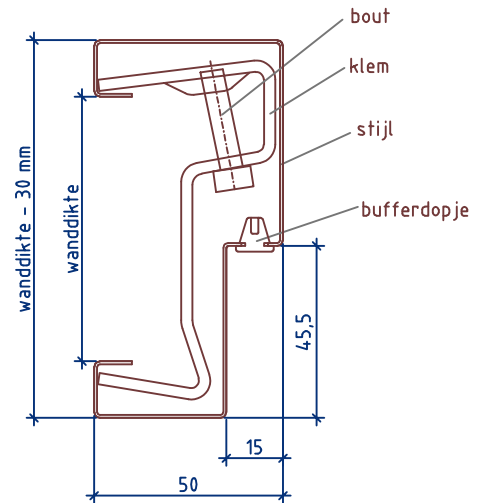
Detail 2: klem
