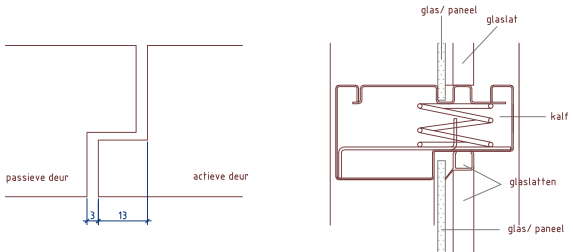
Detail 4: sponning-contrasponning
