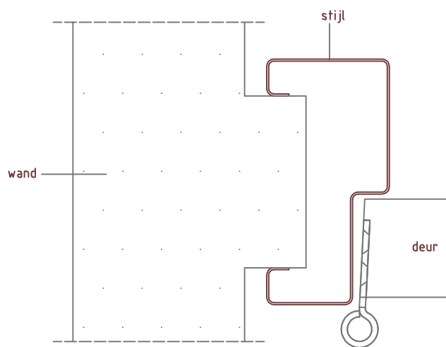
Detail 1: stijl
