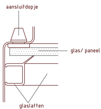
Detail 6: glaslat
