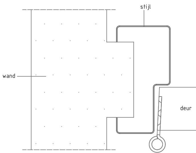
Detail 1: stijl
