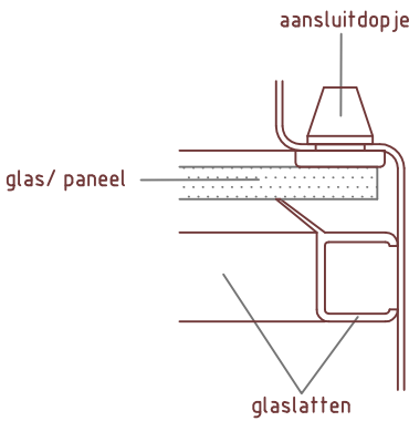
Detail 5: glaslat
