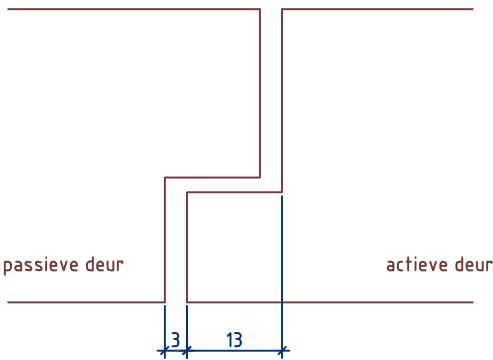
Detail 4: sponning-contrasponning
